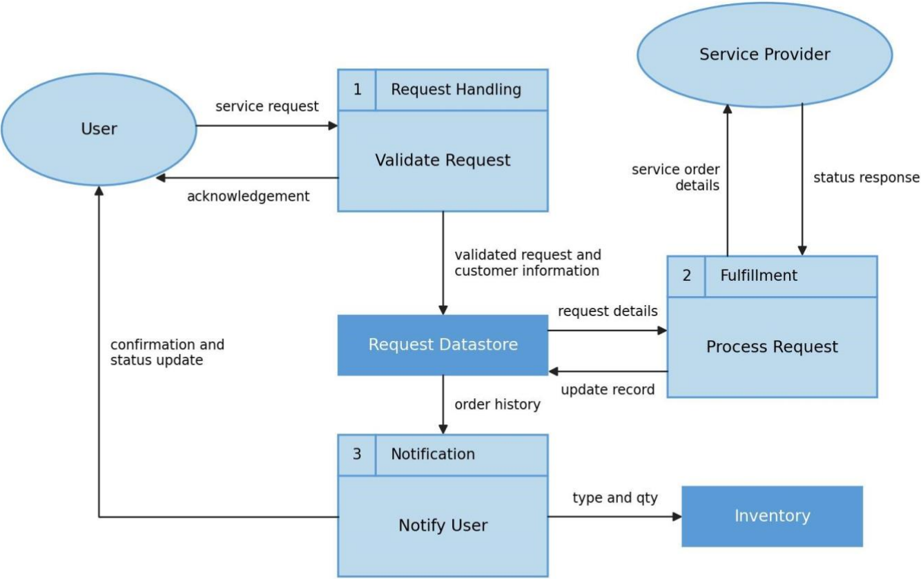
Data Flow Diagram: Online Service Request Management System
